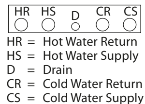
4-pipe
