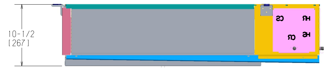
FRONT VIEW
