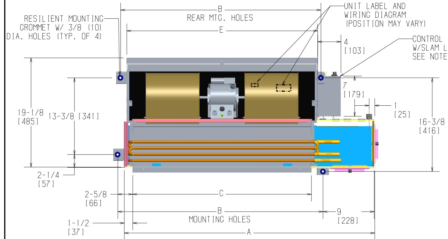
TOP VIEW
