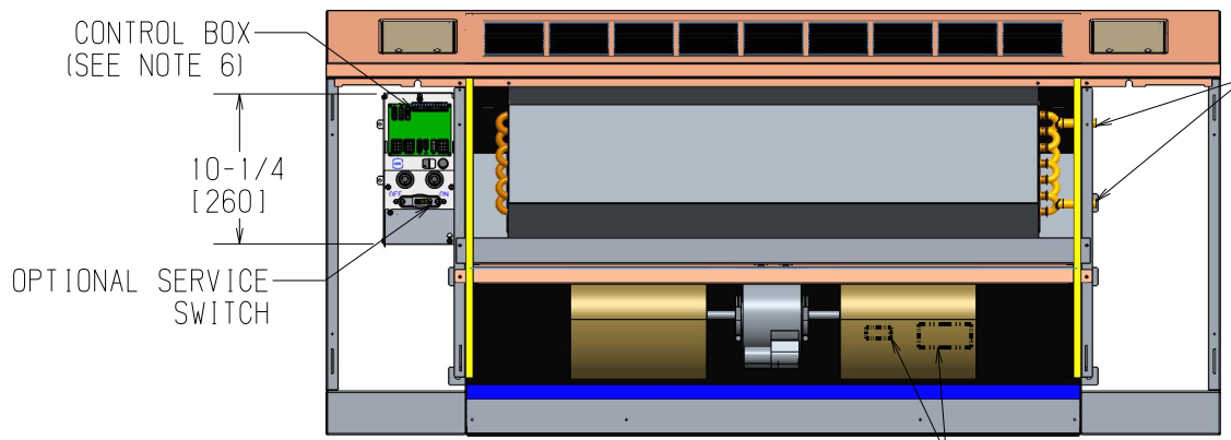
FRONT VIEW (WITHOUT ACCESS PANEL)
