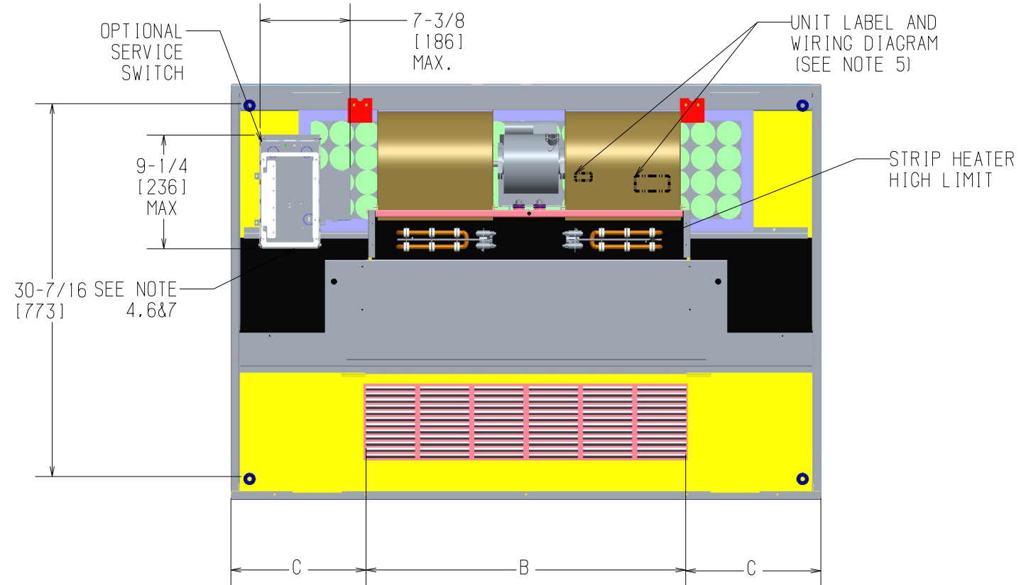
TOP VIEW
