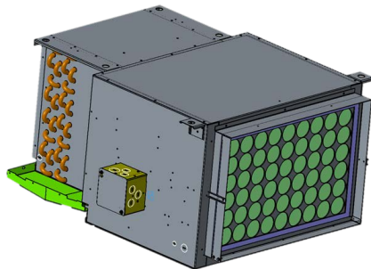
Side Filter Access
